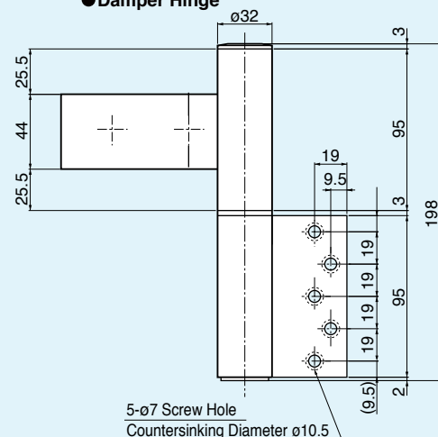
● Damper Hinge
