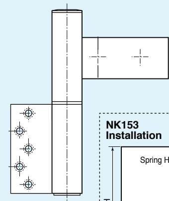
● Damper Hinge
